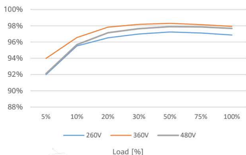
Efficiency Curve
